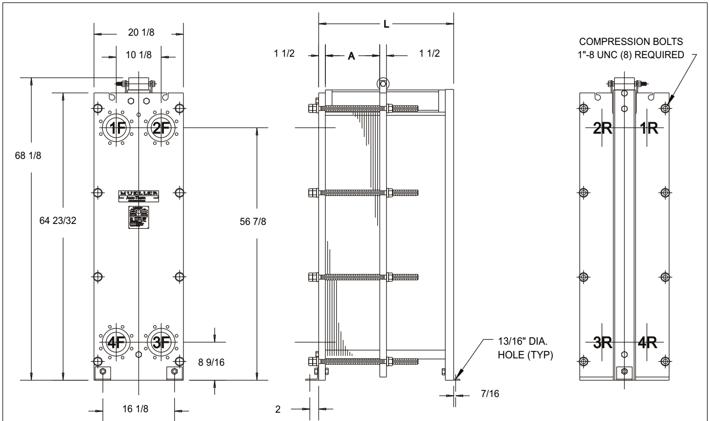
FRONT VIEW
